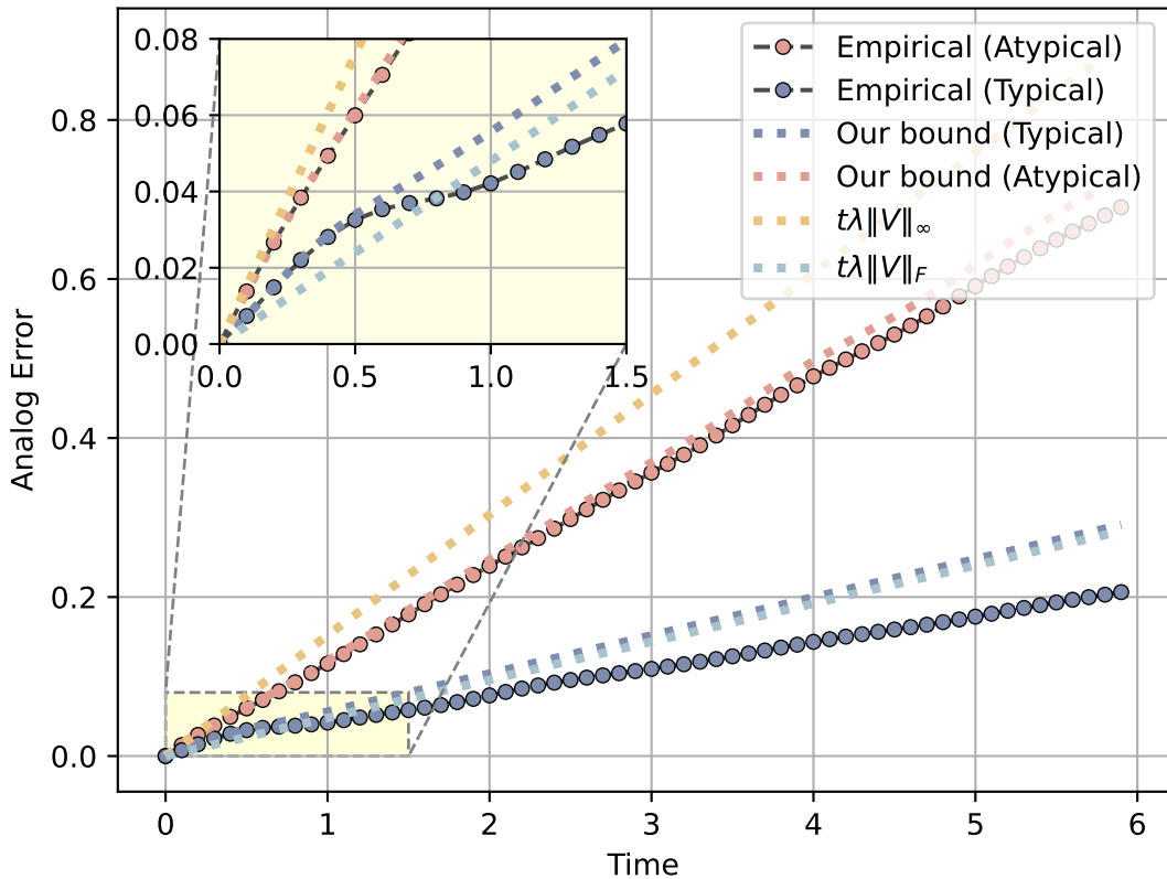
QIMF, long-time evolution with disorder & imperfections
